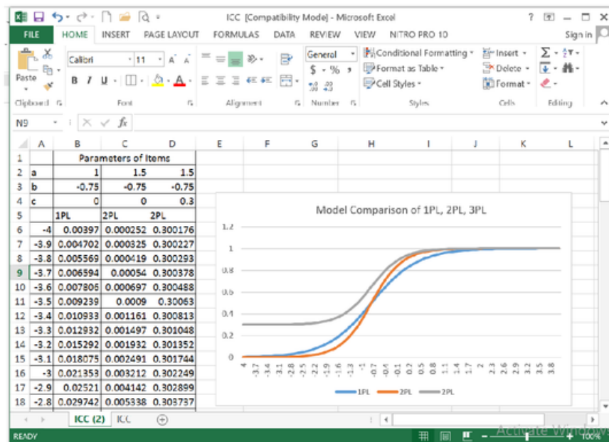
Figure 1. Model Comparison in Unidimensional Item Response Theory
