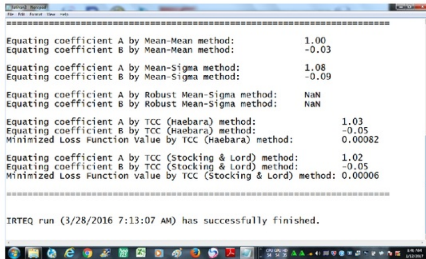
Figure 10. An Example of Analysis Resulted by IRTEQ Program for Generating the Prediction Scores
