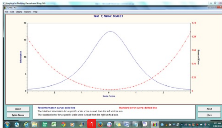
7 Figure 8. An Example of Output from the Value of Item Information Function and Measurement Errors
