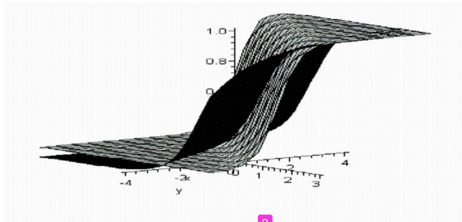
Figure 12. An Example of Item Characteristics Surface for the Focal Group and the Reference Group
