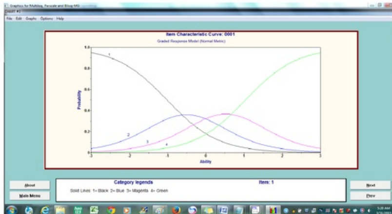
8 Figure 7. An Example of Output from the Item Category Response Function with GRM-Type
